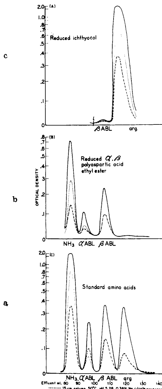
FIG. 8.—Chromatography of lactones obtained from 22-hour hydrolysates of (a) standard amino acids, (b) reduced \alpha,\beta -polyaspartic acid ethyl ester, (c) reduced ichthyocol. The quantity of hydrolysate used corresponded to 1.1 mg for (b) and to 14.5 mg for (c).
